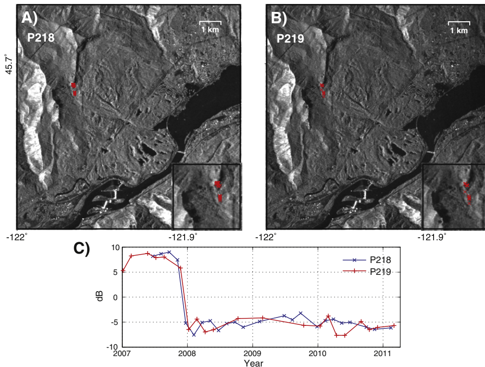
Fig. 5. Detection of the Greenleaf Basin rock avalanche. Averaged amplitude image of P218 (A) and P219 (B) datasets. Red “X”s indicate pixels with dispersion of amplitude larger than 1, consistent with the reported location of the Greenleaf Basin rock avalanche. Insets show the enlarged view of selected pixels. (C) Averaged time-series amplitude of those selected pixels.
