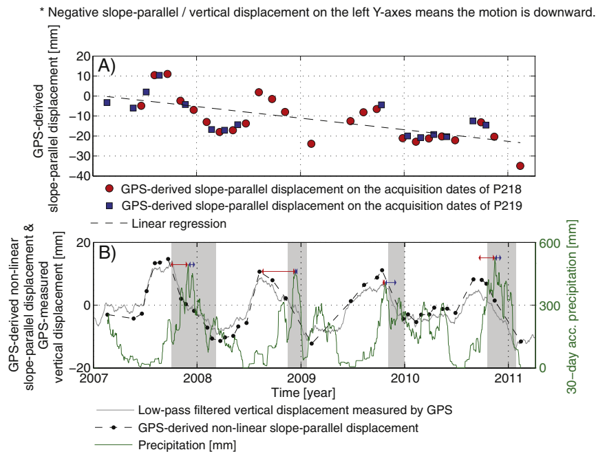
Fig. 10. (A) Regional movement of a nearby GPS station unaffected by landslides is projected into the slope-parallel direction at P to reflect the regional movement component along the slope at this location. (B) GPS-derived non-linear slope-parallel movement (black dashed lines) superposed on the low-pass filtered vertical deformation (gray line), and compared with the 30-day accumulated precipitation total (green line). The difference between this plot and the one in 9 B is that the initiation of downslope motion (black triangles) and the sliding acceleration timespan (gray bars) are determined by the vertical movement measured by GPS, rather than by the non-linear slope-parallel movement obtained from InSAR.
